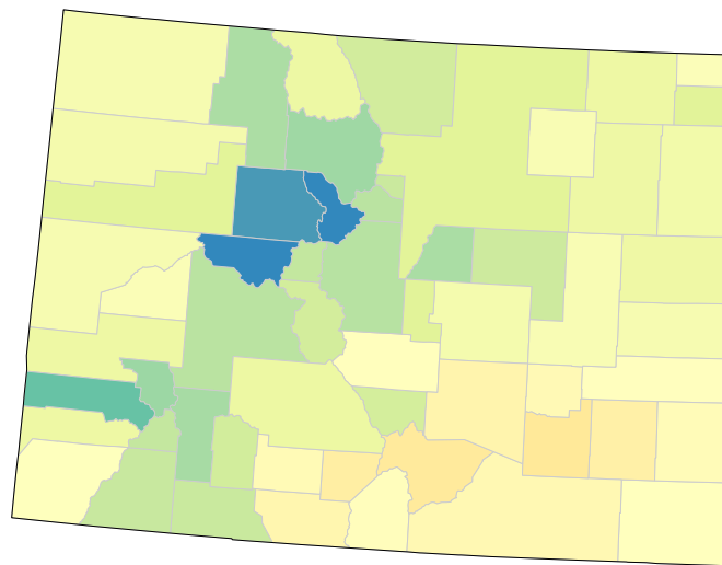
Colorado, life expectancy (years), 2019 65 70 75 80 85 90-93
